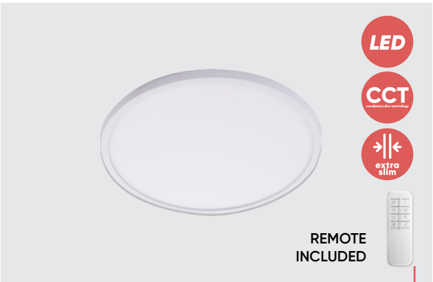
17300 Kraton I. ↑45mm Ø300mm metal, aluminium plastic-matt white LED 18W/1490lm, 2700-6500K EAN 8585032235740 LED G A
