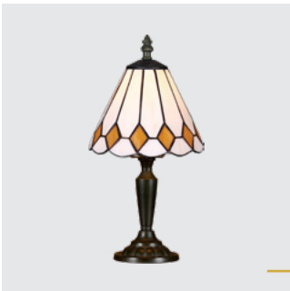
90 Tiffany table ↕320mm ↔160mm ↗160mm metal-antique brown glass-tiffany 1xE14/40W EAN 8585032207648
