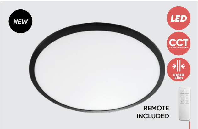
17309 Kraton II. ↑45mm Ø581mm metal, aluminium-matt black plastic-white LED/40W/3200lm, 2700-6500K EAN 858503223775 LED G A
