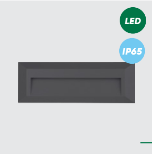
48327 Radix II. ↑80mm ↔230mm ↗27mm plastic-dark grey LED 2.7W/340lm, 4000K EAN 8585032236594 LED IP65
