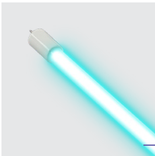
UV 70420 Germicidal tube ↓15mm ↔589mm ↗15mm T5 UV-C/14W EAN 8585032236556 Ⓟ Ⓢ Ⓣ
