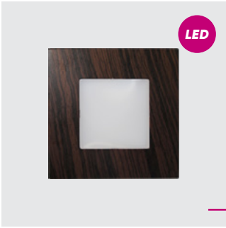
48306 Step light 86mm x 86mm x 35mm plastic-dark wood LED 1W/60lm, 4000K EAN 8585032221514
