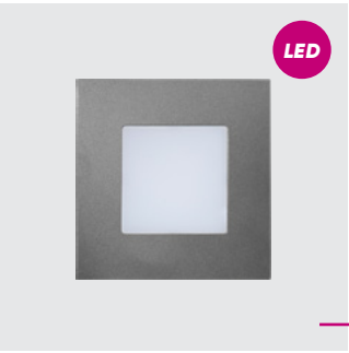
48305 Step light 86mm x 86mm x 35mm plastic-anthracite LED 1W/60lm, 4000K EAN 8585032221507
