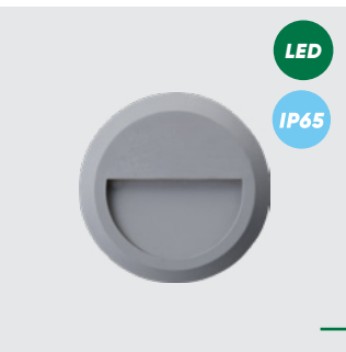
48314 Radix I. ↑150mm ↔150mm ↗27mm plastic-grey LED 1.5W/190lm, 4000K EAN 8585032221590 LED IP65
