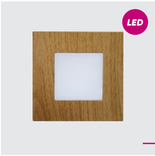
48307 Step light 86mm x 86mm x 35mm plastic-light wood LED 1W/60lm, 4000K EAN 8585032221521
