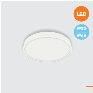
49035 Lenys II. Ø25mm Ø140mm metal-white plastic-white LED 12W/1200lm, 4000K EAN 8585032236303 LED IP20 IP44 LED F A G
