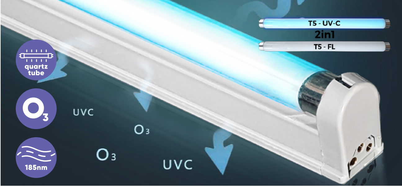
UV 70421 Germicidal tube ↓15mm ↔1163mm ↗15mm T5 UV-C/28W EAN 8585032236563 Ⓟ Ⓢ Ⓣ
