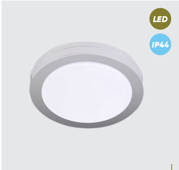
48605 Downlight ↓48mm Ø82mm iron-chrome abs-white LED 6W/500lm, 4000K EAN 8585032235900 LED
