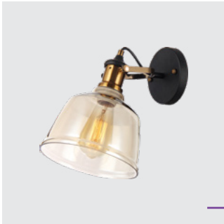
46307 Famosa III. ↓250mm ↔190mm ↗250mm metal-black/antique brass, glass-cognac 1xE27/40W EAN 8585032234316 ⓔ27 Ⓛ Ⓢ
