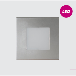
48302 Step light 86mm x 86mm x 35mm plastic-silver LED 1W/60lm, 4000K EAN 8585032216008
