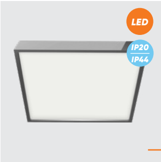
49053 Lenys SQ I. Ø25mm ↔280mm 280mm metal-chrome plastic-white LED 30W/3420lm, 4000K EAN 8585032237409
