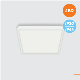
49040 Lenys SQ II. Ø25mm ↔190mm 190mm metal-white plastic-white LED 18W/1800lm, 4000K EAN 8585032236358 LED IP20 IP44 LED F A G
